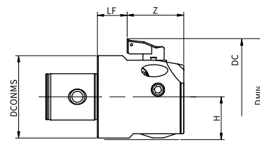
Min. through hole diameter DMIN = H+(Back-boring diameter/2)
