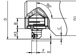
B-type Fine Adjustment Cartridge--- Perpendicular installation
