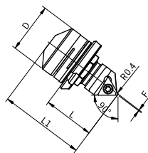
A-type Fine Adjustment Cartridge-- installation with an angle
