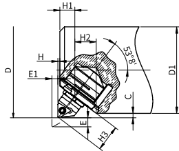
A-type Fine Adjustment Cartridge--- Installation with an angle
