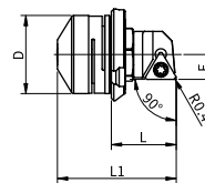
B-Type Fine Adjustment Cartridge--- perpendicular installation
